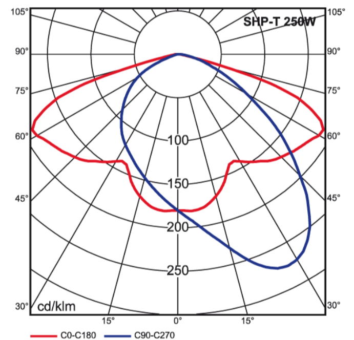
Distribution curve for LUNOIDA S-250W luminaire
